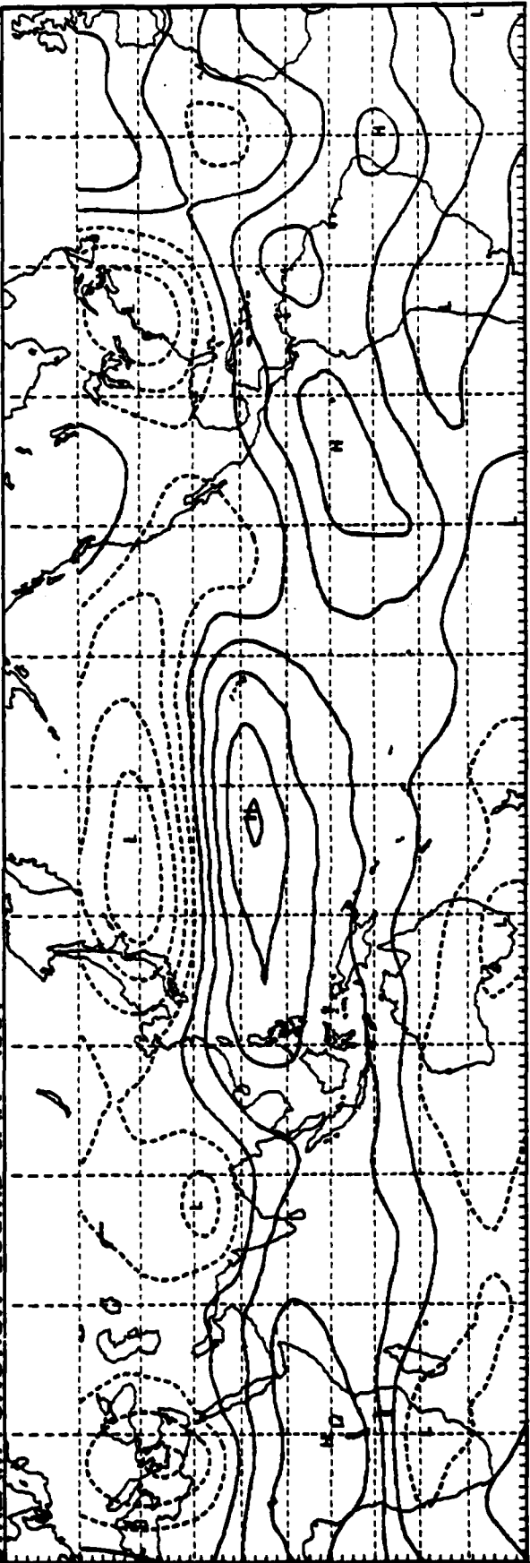
STREAM FUNCTION 200MB JAN 1981
